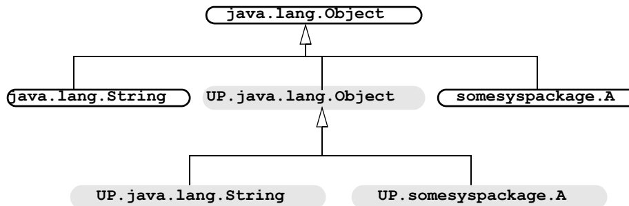
Figure 1(b): Replicating system classes in a user package (“UP”)
