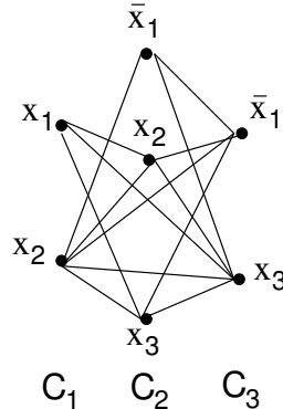
Figure 17.6 The graph generated from Boolean expression B = (x_1 + x_2) \cdot (\bar{x}_1 + x_2 + x_3) \cdot (\bar{x}_1 + x_3) . Literals from the first clause are labeled C1, and literals from the second clause are labeled C2. There is an edge between every pair of vertices except when both vertices represent instances of literals from the same clause, or a negation of the same variable. Thus, the vertex labeled C1 : y_1 does not connect to the vertex labeled C1 : y_2 (because they are literals in the same clause) or the vertex labeled C2 : \bar{y}_1 (because they are opposite values for the same variable).
