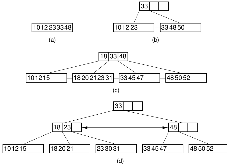
Figure 10.18 Examples of B + -tree insertion. (a) A B + -tree containing five records. (b) The result of inserting a record with key value 50 into the tree of (a). The leaf node splits, causing creation of the first internal node. (c) The B + -tree of (b) after further insertions. (d) The result of inserting a record with key value 30 into the tree of (c). The second leaf node splits, which causes the internal node to split in turn, creating a new root.
