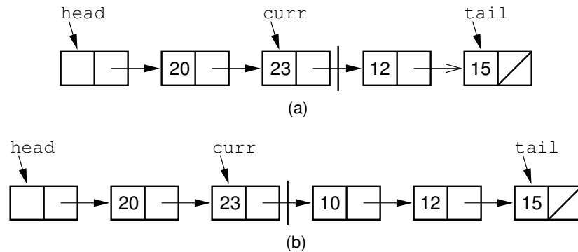
Figure 4.7 Insertion using a header node, with curr pointing one node head of the current element. (a) Linked list before insertion. The current node contains 12. (b) Linked list after inserting the node containing 10.
