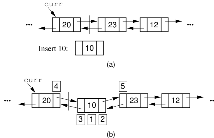
Figure 4.15 Insertion for doubly linked lists. The labels 1 , 2 , and 3 correspond to assignments done by the linked list node constructor. 4 marks the assignment to curr->next . 5 marks the assignment to the prev pointer of the node following the newly inserted node.
