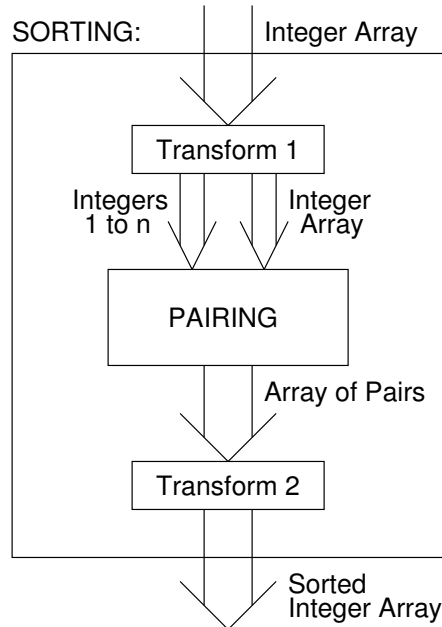
Figure 17.3 The reduction of SORTING to PAIRING shown as a “blackbox” diagram.
