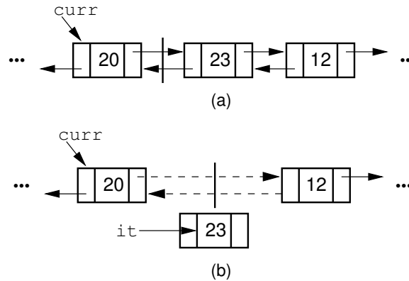
Figure 4.16 Doubly linked list removal. Element it stores the element of the node being removed. Then the nodes to either side have their pointers adjusted.
