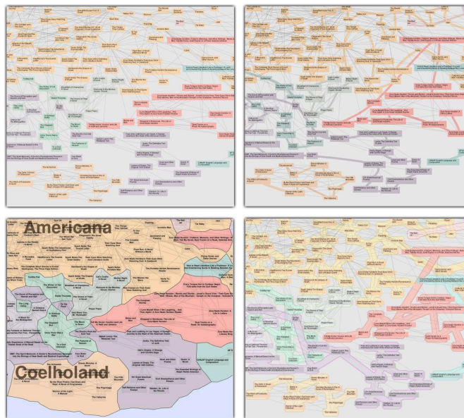
Fig. 5. Four options for displaying cluster membership as studied by Jianu et al [51]. In addition to a node-link representation similar to that included by Saket et al., this study included Linesets [5], GMap [41], and BubbleSets [24].
