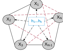
Fig. 4: Original Method (ARX + ARXL) Invariant Graph
