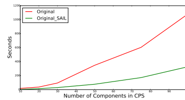
Fig. 25: Running Time of Original (ARX + ARXL) vs. Original (ARX+ARXL) + SAIL
