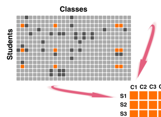
Fig. 1. An example of a bicluster extracted from a students-to-classes relation. Dark cells indicate existing relationships, and orange cells represent relationships part of this bicluster. Three students took the same four classes.
