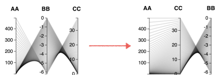
Fig. 5. An example of rearranging axes by switching axes BB and CC 4 .
