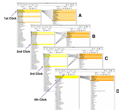
Fig. 4. An example of finding a bicluster in Jigsaw's List View. Yellow indicates entities that a user selected and orange indicates relevant entities corresponding to the selected one(s) based on word co-occurrence.
