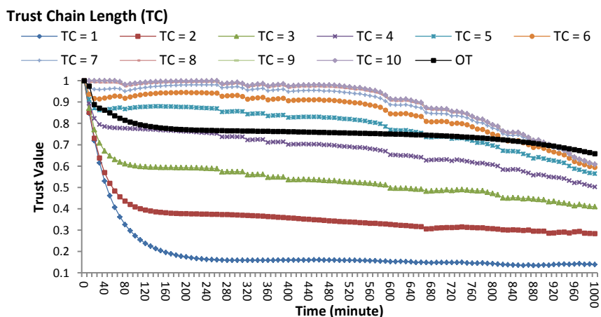
Fig. 2. Trust value vs. length of a trust chain (TC) over time: one node’s evaluation toward another node.
