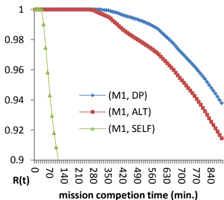
Fig. 7. A node's trust-based reliability R(t) over time under M1 under various behavior models.
