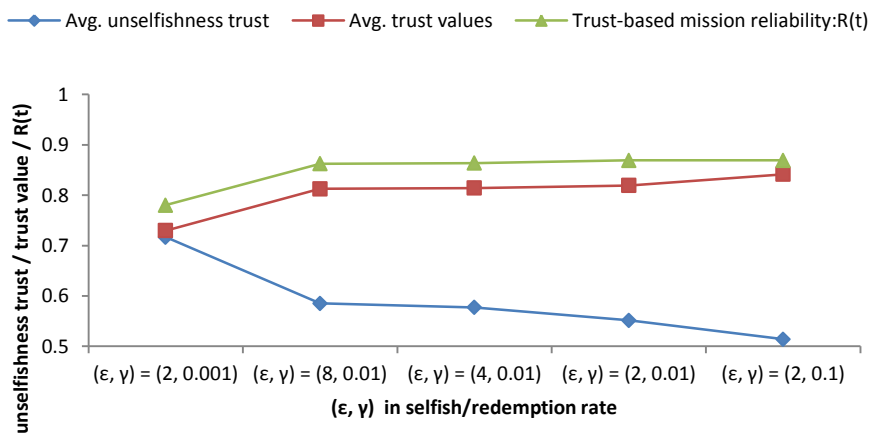
Fig. 13. Impact of (\epsilon, \gamma) on unselfishness trust, overall trust and mission reliability.
