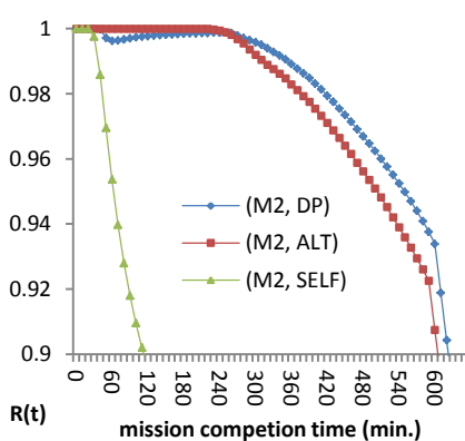
Fig. 8. A node's trust-based reliability R(t) over time under M2 under various behavior models.
