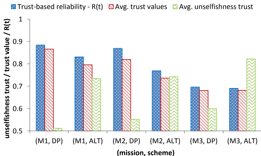
Fig. 10. A comparative performance analysis of DP vs. ALT over all mission scenarios.
