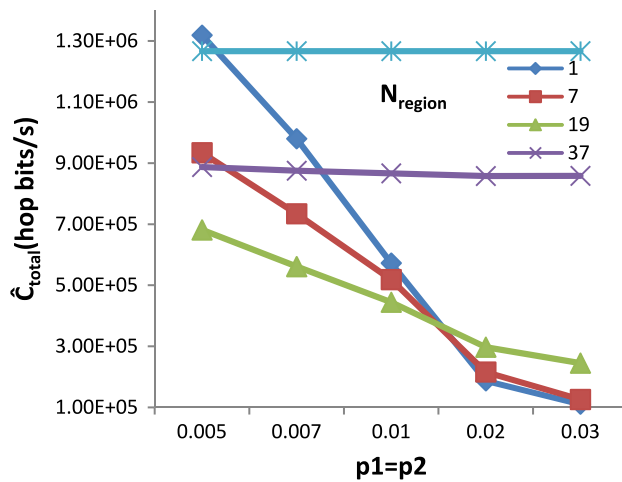
Fig. 8. \hat{C}_{total} versus p1 and p2 with varying N_{region} .
