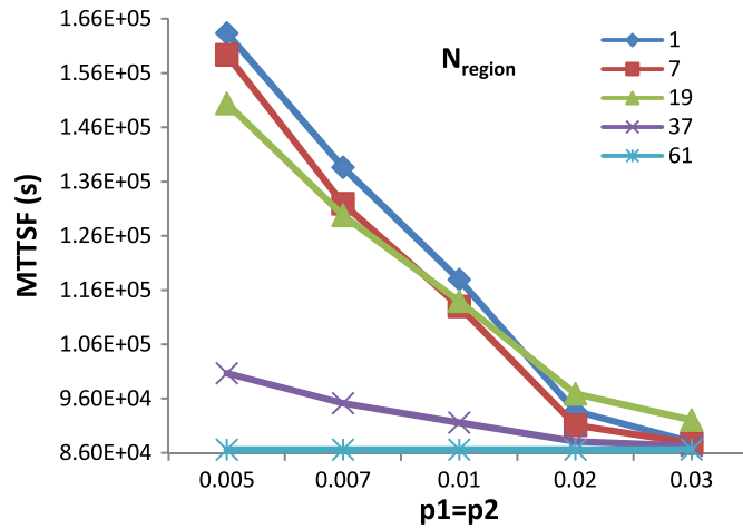
Fig. 7. MTTSF versus p1 and p2 with varying N_{region} .
