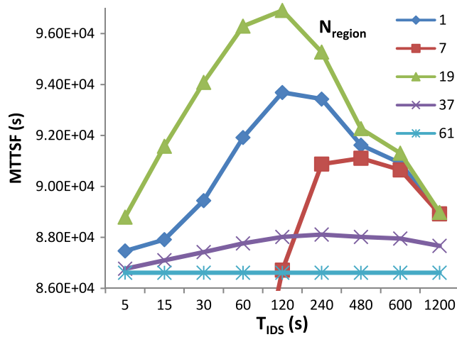
Fig. 5. MTTSF versus T_{IDS} with p_1 = p_2 = 0.02 .
