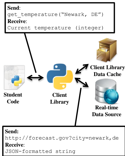
Figure 1: Client Library Architecture
