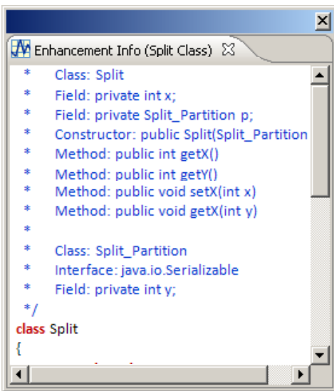
Figure 16. Documentation for the Split class Enhancement.
