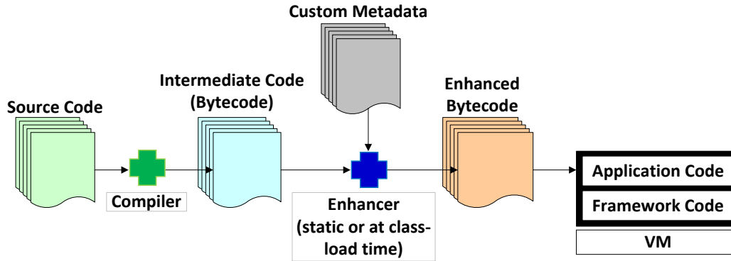
Figure 1. Enhancing intermediate code via bytecode engineering.
