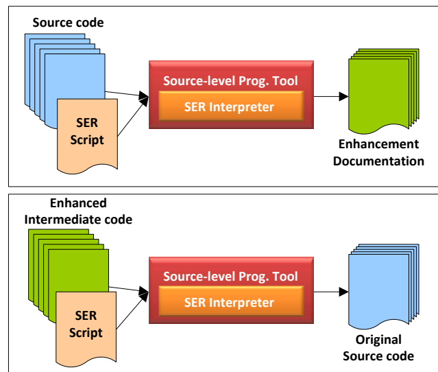
Figure 4. Source level programming tools with intermediate code enhancement information.
