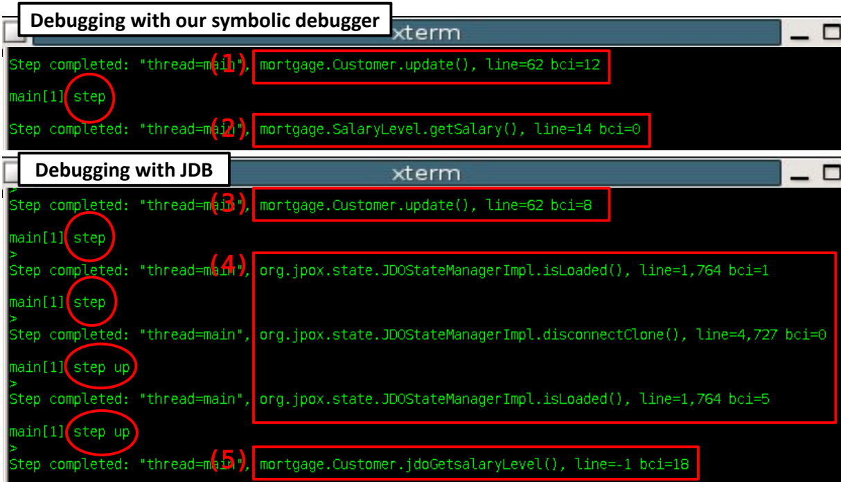
Figure 20. Debugging enhanced code: Debugger with an enhancements awareness vs. JDB
