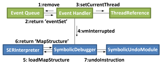
Figure 19. The symbolic debugger’s collaboration diagram.
